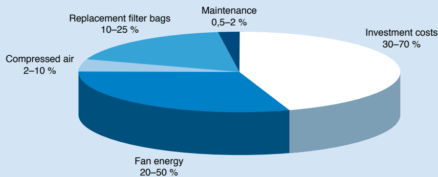
Total cost of ownership of IMPULS filtration plants over an operating period of 10 years
