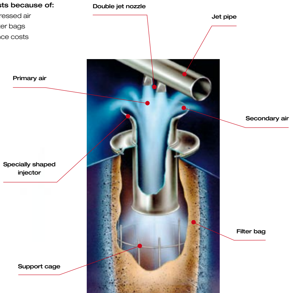
Patented IMPULS cleaning system
